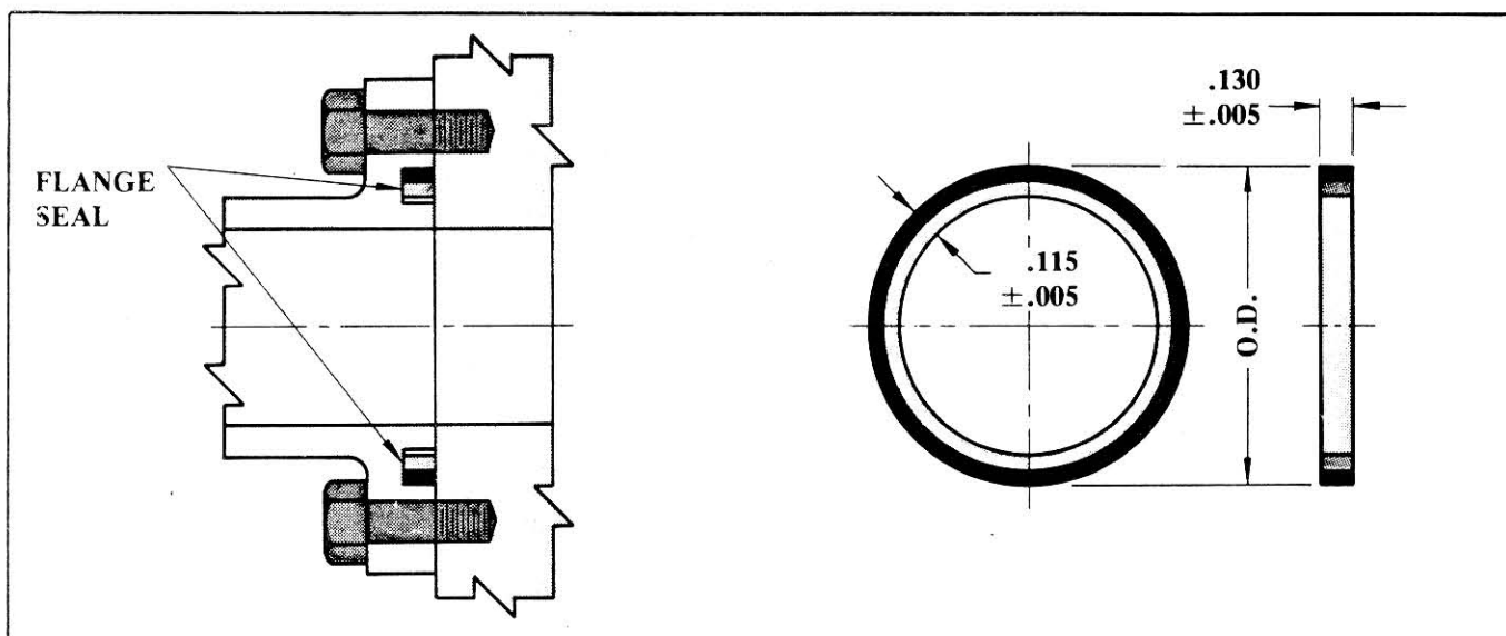
SIZES FOR SAE J518c 4 BOLT SPLIT FLANGE TYPE CONNECTIONS
